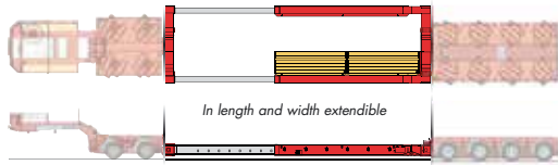
Vessel bed with detachable wooden floor
